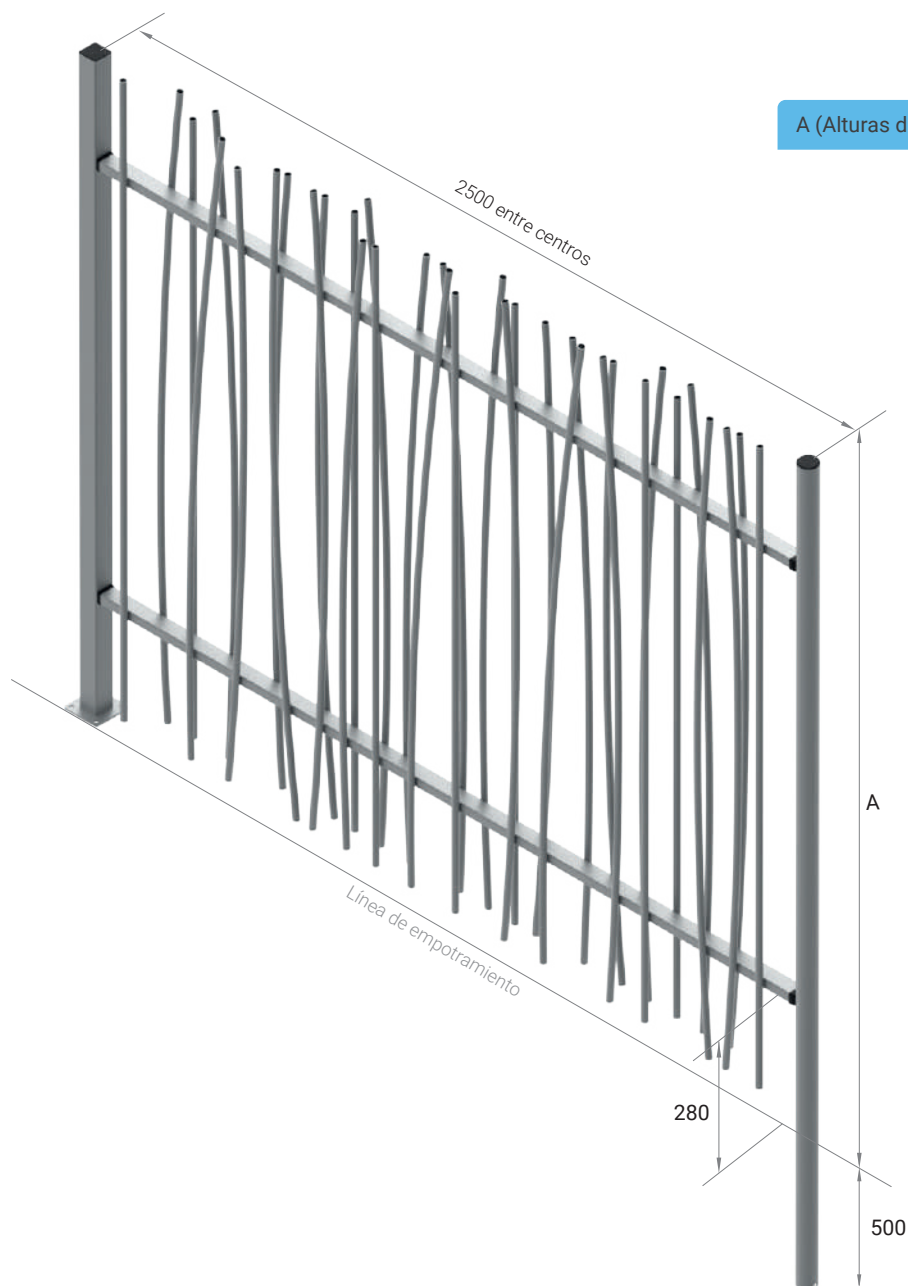
Detalle barros Brote
