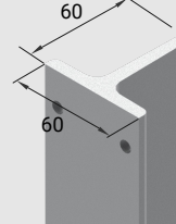
Riostra Simple T 60 x 7 mm
